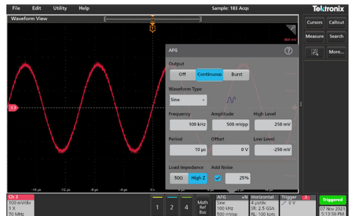
Flexible settings of AFG outputs. In this test case, 25% of noise was added to the Sine.
